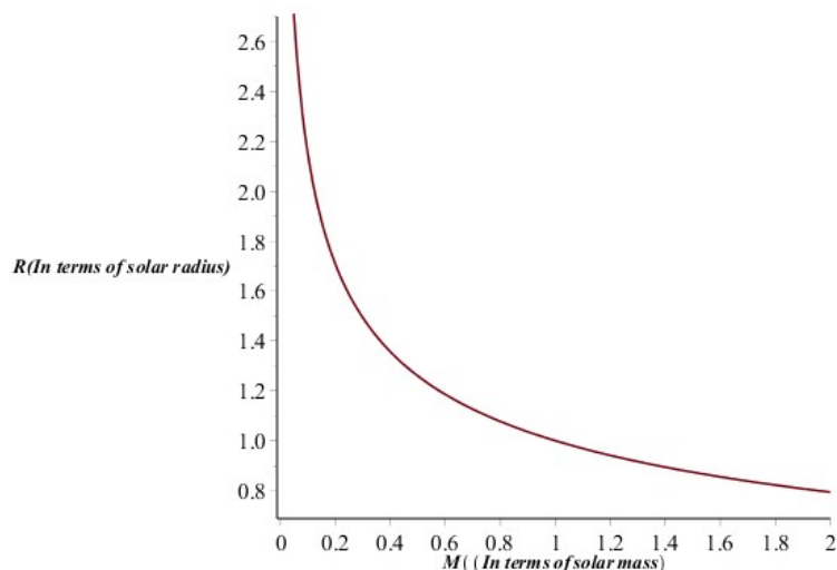
Fig. 1 Radius versus mass plot for a white dwarf, showing that its size decreases as its mass increases. (The axes of the plots are in terms of the solar radius R_{\odot} = 6.960 \times 10^8 m , and the solar mass M_{\odot} = 1.98892 \times 10^{30} kg .)
