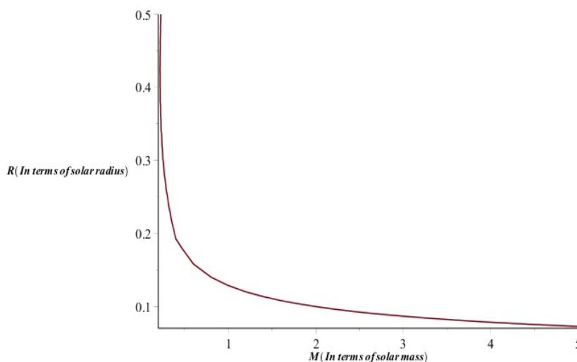
Fig. 4 Radius versus mass diagram of a white dwarf with EUP correction. (The axes of the plots are in terms of the solar radius R_{\odot} = 6.960 \times 10^8 m and the solar mass M_{\odot} = 1.98892 \times 10^{30} kg .)
