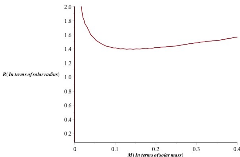
Fig. 2 Radius versus mass plot for a white dwarf with GUP correction. Initially, the size of the white dwarf decreases with increasing mass, then it recovers and can grow to an unlimited size. (The axes of the plots are in terms of the solar radius
