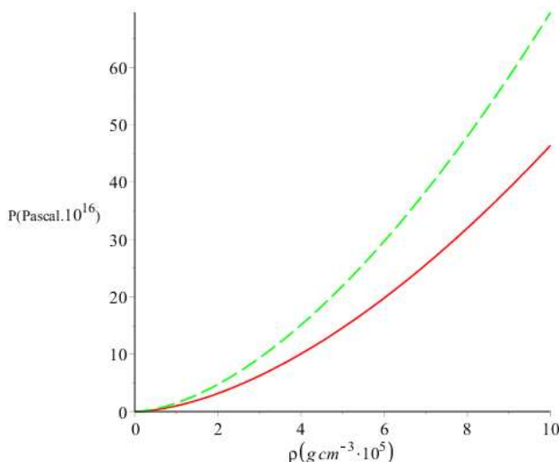
Fig. 5 Pressure p versus density \rho for a white dwarf (red diagram for the standard state and green (dashed line) considering EUP).
