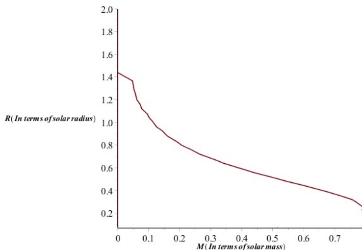
Fig. 3 Radius versus mass plot of a white dwarf incorporating the Generalized Uncertainty Principle (GUP) correction with a negative parameter. (The axes of the plots are in terms of the solar radius R_{\odot} = 6.960 \times 10^8 m and the solar mass M_{\odot} = 1.98892 \times 10^{30} kg .)
